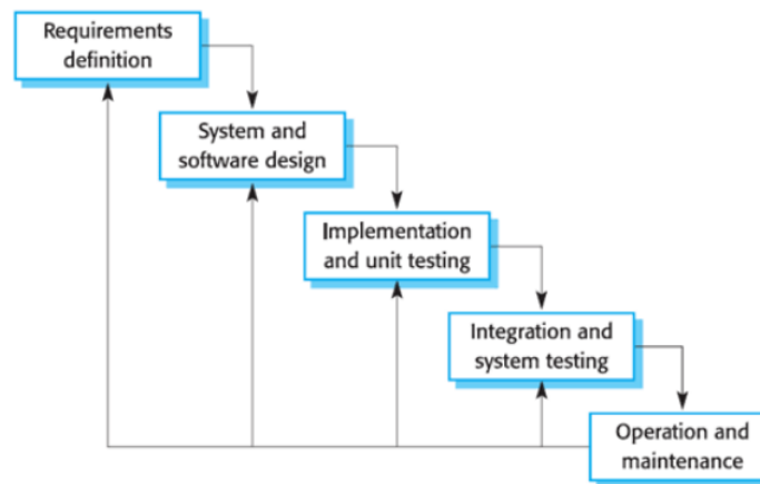
Figure 1. Waterfall method
