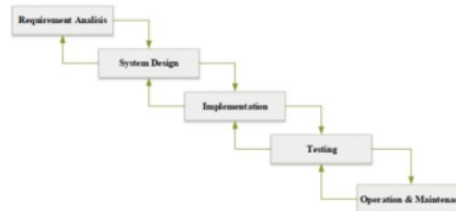
Gambar 4 Waterfall Diagram
