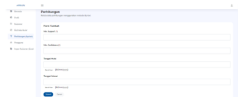
Gambar 7. Perhitungan Apriori
