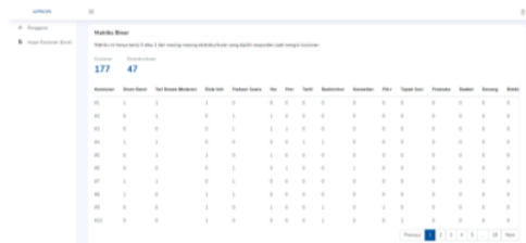
Gambar 8. Matrik biner
