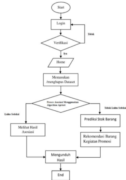
Gambar 3. Flowchart Sistem
