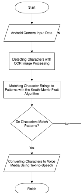
Fig 1. Flowchart of the Knuth-Morris-Pratt Algorithm Application System on Android Applications for Recognition of Nominal Money for the Blind
