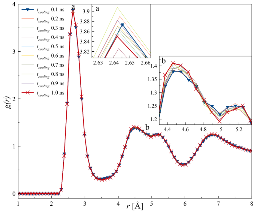
Figure 3. The radial distribution function g(r) of the NiTi alloy after the solidification process over a number of different variations of the cooling rate. (a) The first peak of the radial distribution function g(r) ; (b) The second and shoulder peaks of the radial distribution function g(r) .
