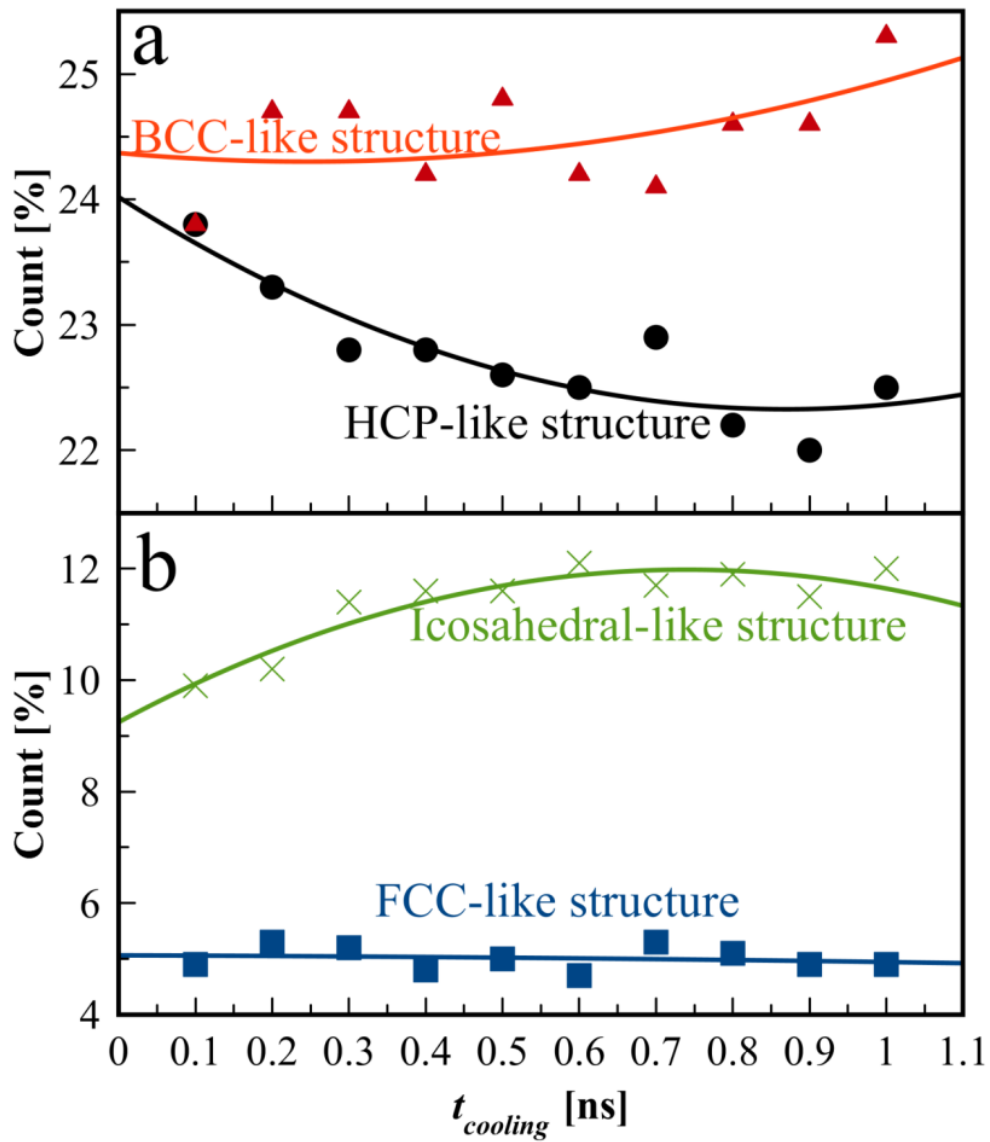
Figure 4. Local structure analysis of glassy NiTi alloy at low temperature of 10 K for (a) BCC- and HCP-like structure, and (b) Icosahedral- and FCC-like structure.
