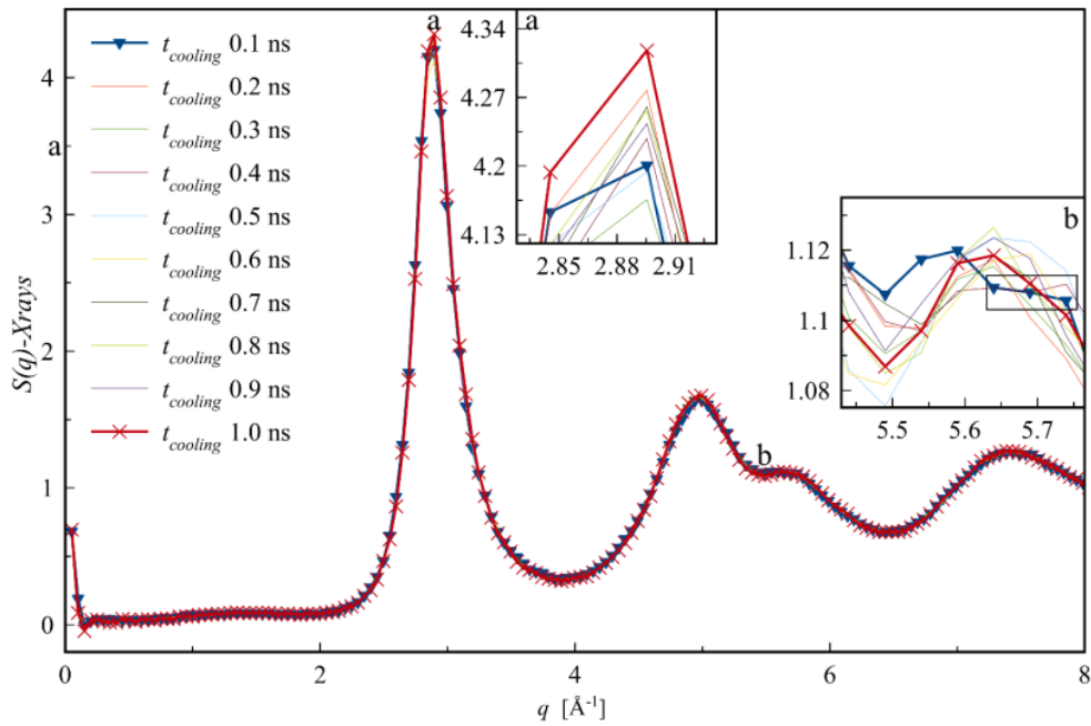
Figure 2. The structure factor S(q) of the NiTi alloy after the solidification process over a number of different variations of the cooling rate. (a) The first peak of the glassy NiTi structure factor; (b) the shoulder of the second peaks of structure factor of glassy NiTi.
