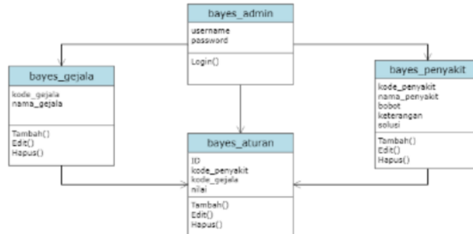
Gambar 3. Class Diagram
