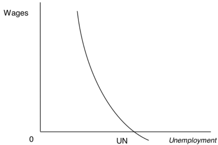
Gambar 1. Kurva Phillips
