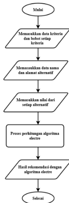
Gambar 1: Flowchart Sistem
