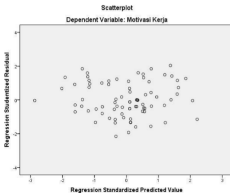
Gambar 2. Scatter Plot Uji Heteroskedastisitas
