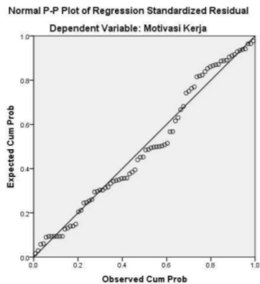
Gambar 1. Diagram Plot Uji Normalitas
