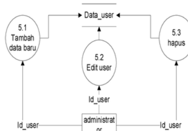
Gambar DFD level 2 Data User
