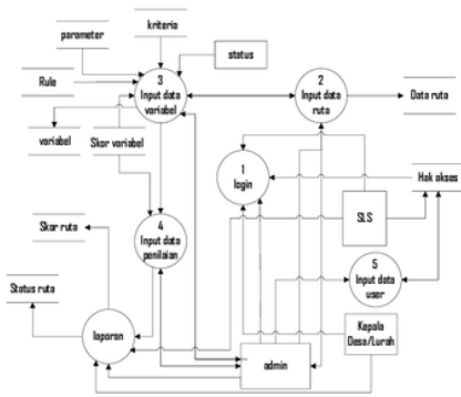
Gambar DFD level 1
