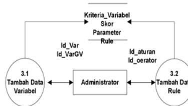
Gambar DFD level 2 Administrator
