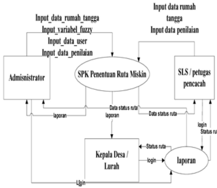
Gambar DFD level 0
