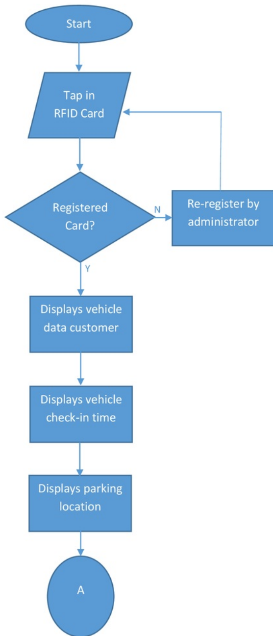
Figure 3. Flowchart of System 1
