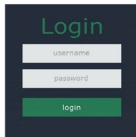
Figure 6. Login Form
