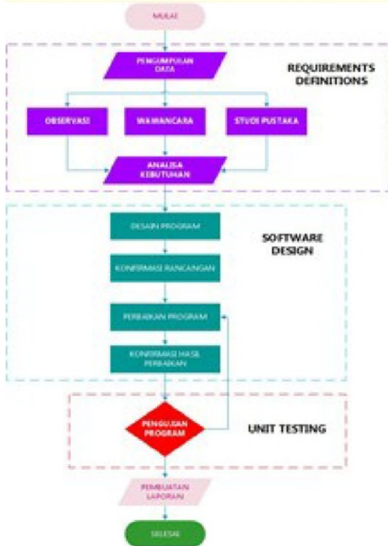
Figure 1. Waterfall Methodology
