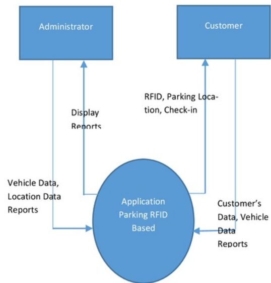
Figure 5. The DFD Parking System
