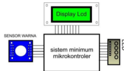
Gambar 3.1 Diagram Blok
