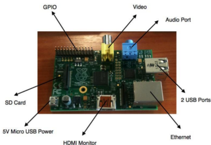
Gambar 1. Raspberry Board
