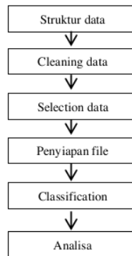
Gambar 1. Sistematika Penelitian [7]
