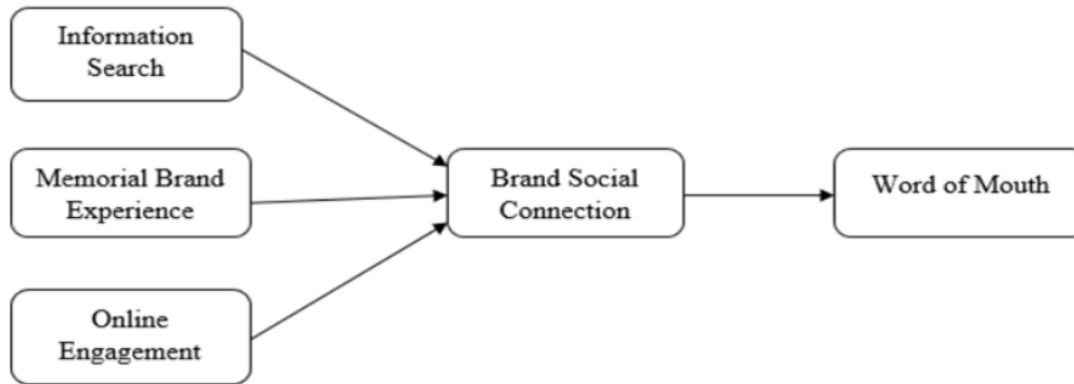
Figure 3: Conceptual Model
