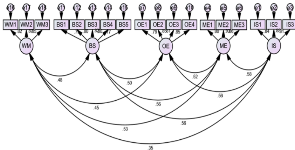
Figure 4: CFA
