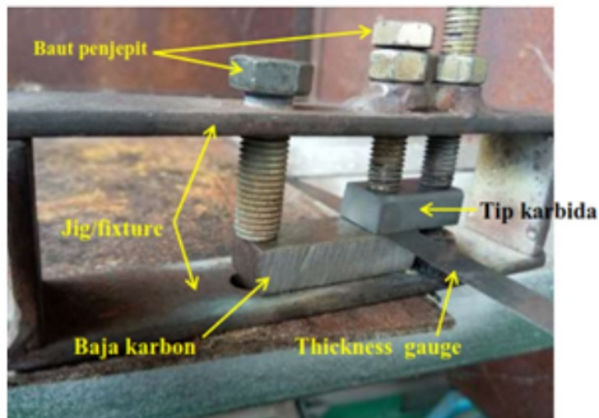
Figure 2. Jig/fixture
