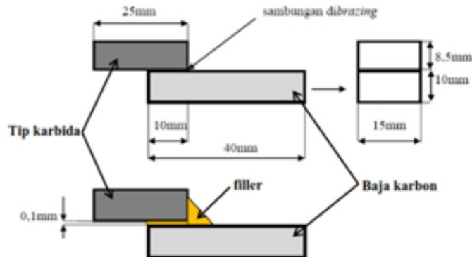
Figure 1. Skema sambungan
