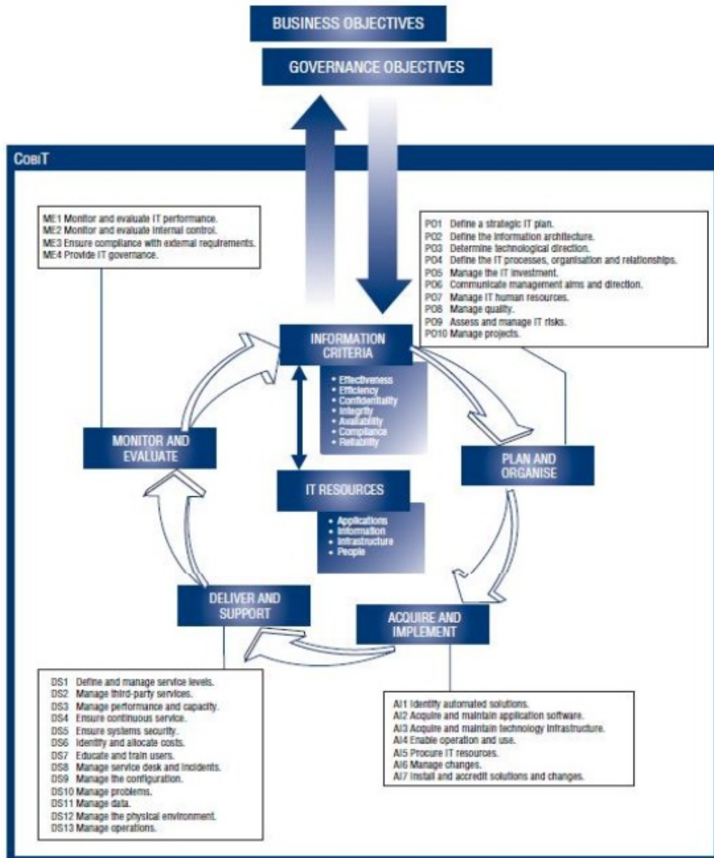
Gambar 8.1. Framework COBIT 4.1
