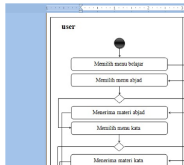
Gambar 3 Activity Diagram Belajar
