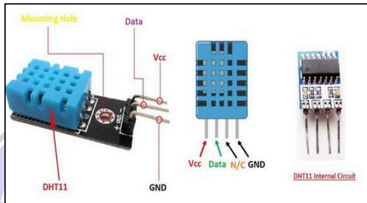
Gambar 2.3 Sensor DHT11
