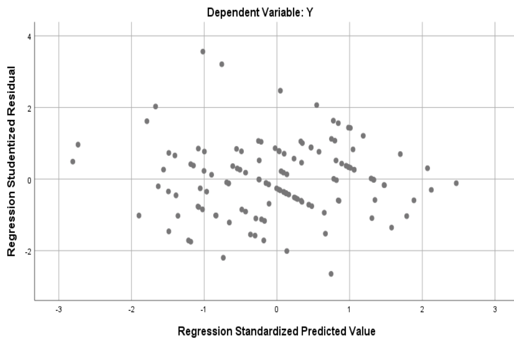
Scatterplot
