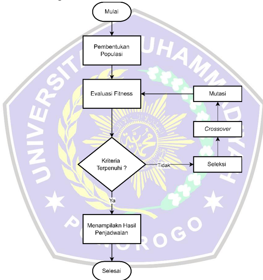
Gambar 2. Flowchart Algoritma Genetika
