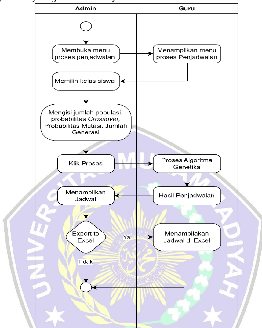
Gambar 4. Activity Diagram Proses Penjadwalan
